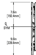
SIDE VIEW RETRACTED
