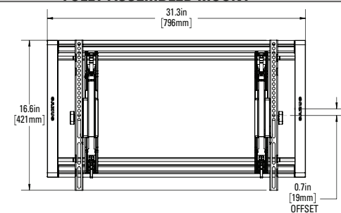
FULLY ASSEMBLED MOUNT
