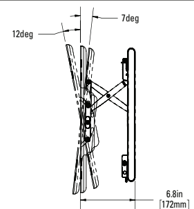
SIDE VIEW RETRACTED
