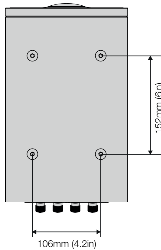
CABINET BASE STAND SCREW ALIGNMENT
